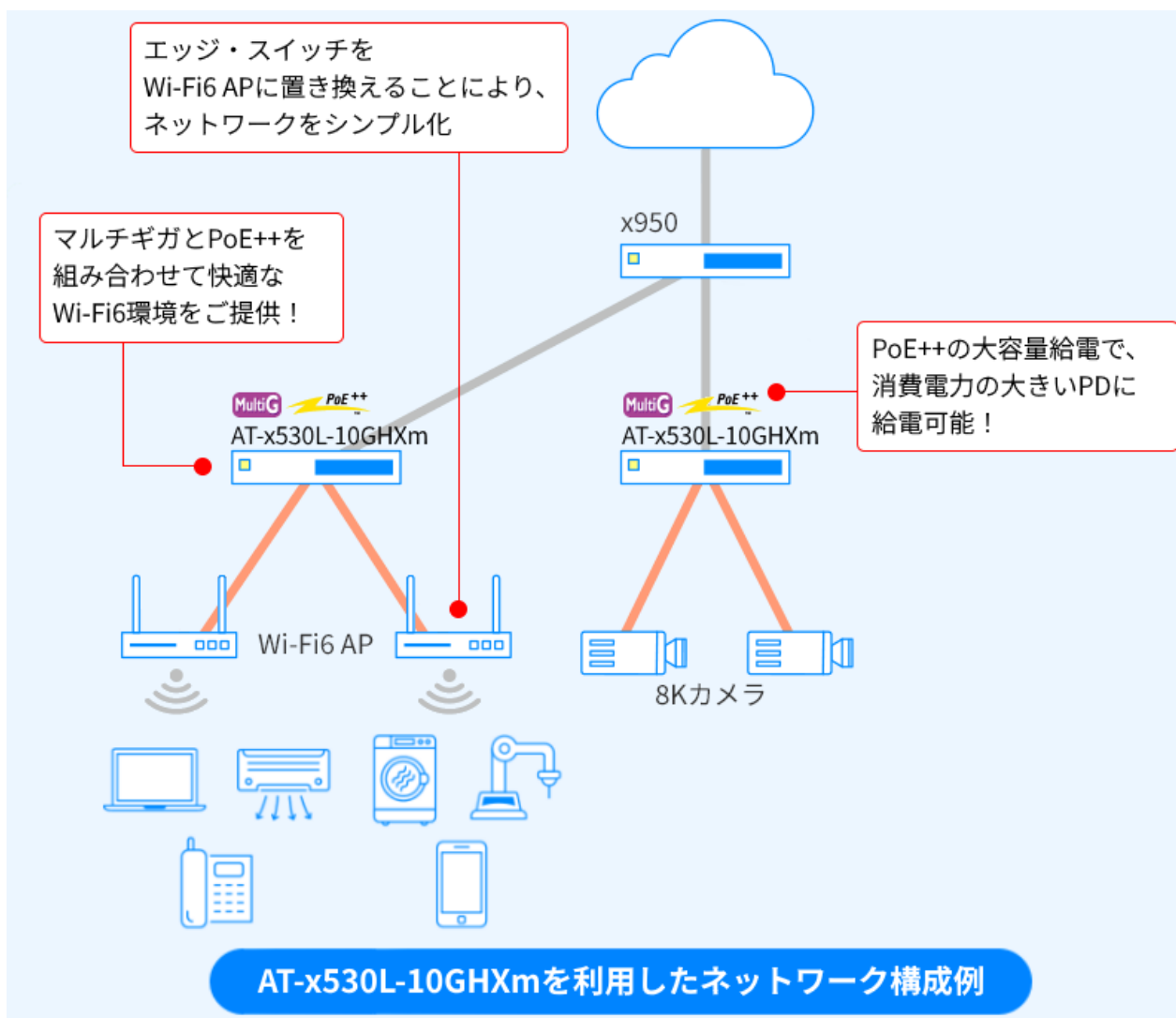
AT-x530L-10GHXm
